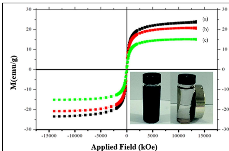
Figure 4. VSM plot for (a) Fe 3 O 4 (24.48 emu/g), (b) NH 2 -SiO 2 /Fe 3 O 4 (20.10 emu/g), (c) alg/Cs-NH 2 -SiO 2 /Fe 3 O 4 (14.77 emu/g). The photo showed the separation of adsorbent using an external magnet.
