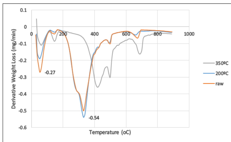
Figure 6. Derivative weight loss of raw dry leaves and bio-coal at different temperatures
