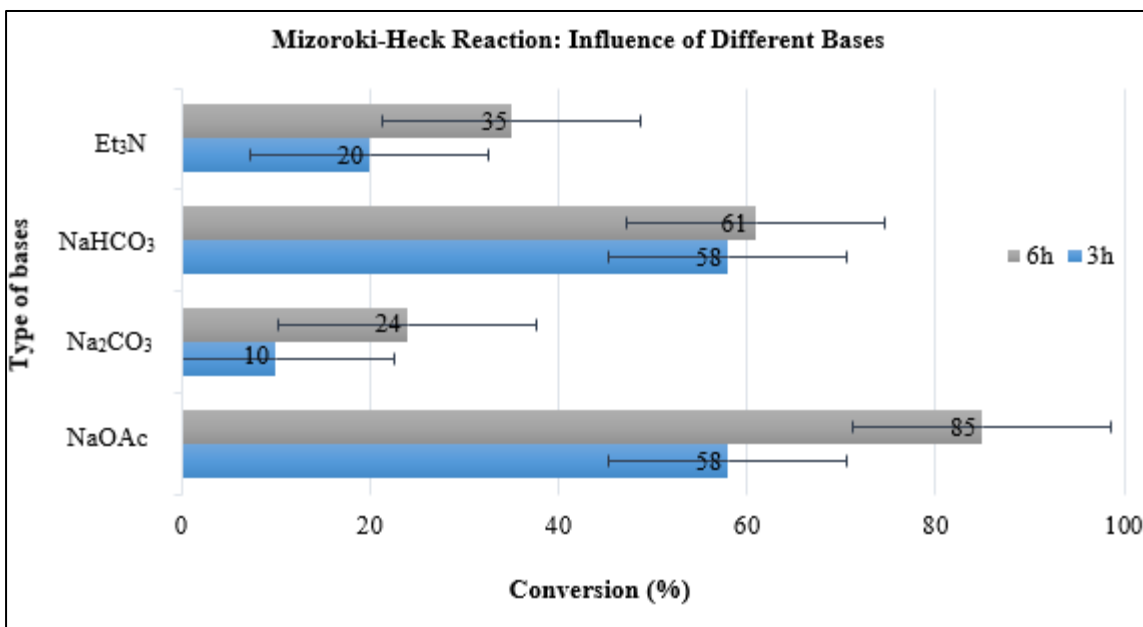
Figure 1. Results obtained for Mizoroki-Heck reaction with a different type of bases
